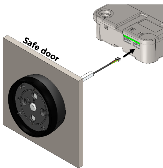
Standard version (p.n T6550)
