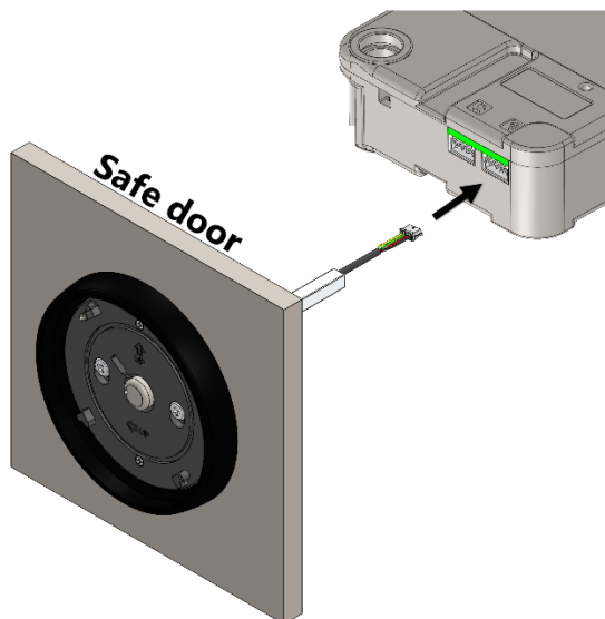
Flat version (p.n T6540)
